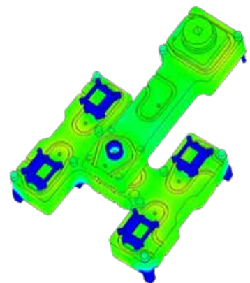
Fig. 2 Optimal thermal distribution ensures the right balance between polymer behavior and part quality.
