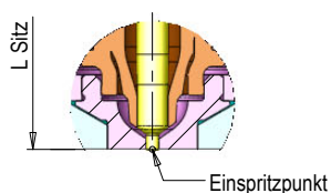
Version L=11
