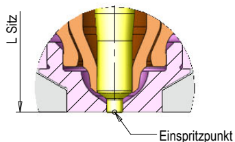
Version L=13
