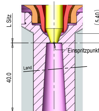
Version L=82
