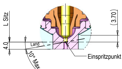
Version L=15
